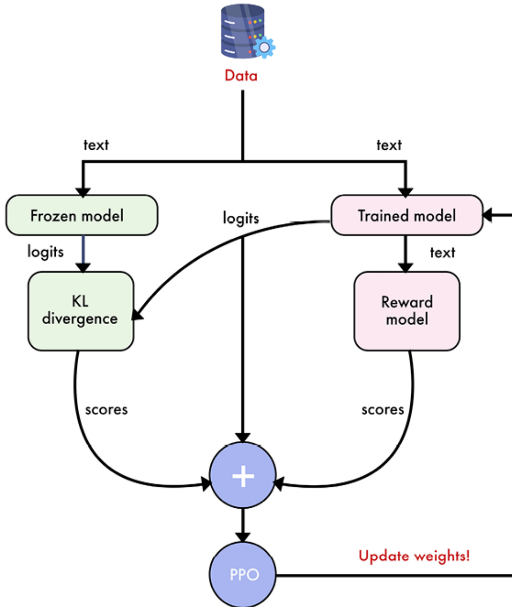
Figure 6.4 – High-level view of the PPO algorithm for preference alignment
