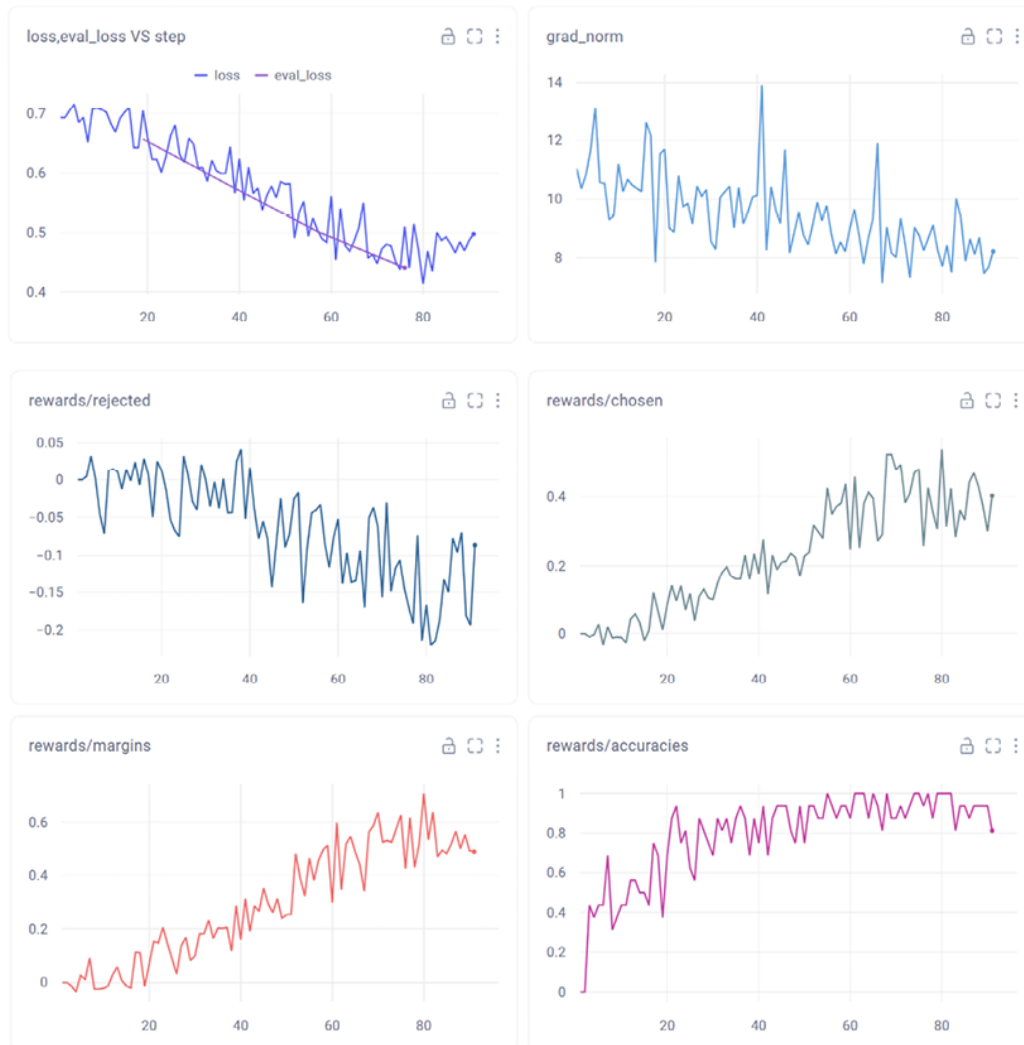
Figure 6.6 – Experiment tracking in Comet ML with DPO metrics
